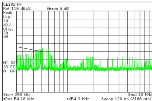
Fig. 14: CE102 high frequency band scan
