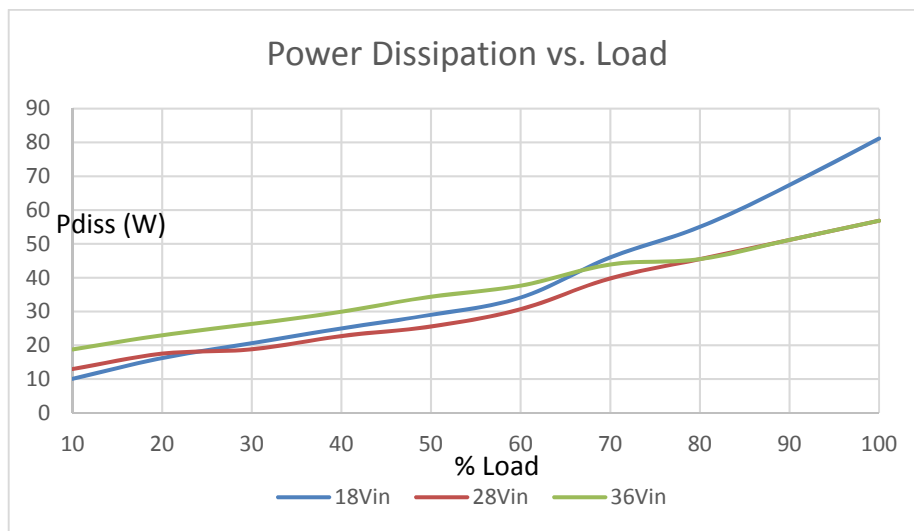
Figure 83: Power dissipation vs. Load for Minimum, Nominal and Maximum input voltage
