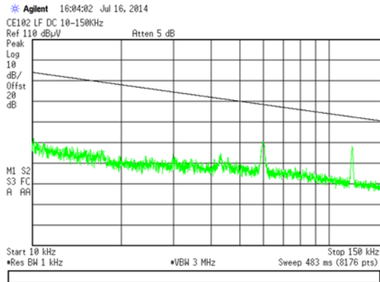
Figure 11: CE102 low frequency band scan
