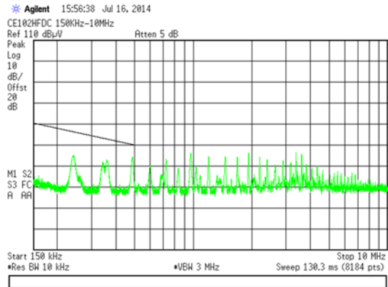
Figure 12: CE102 high frequency band scan
