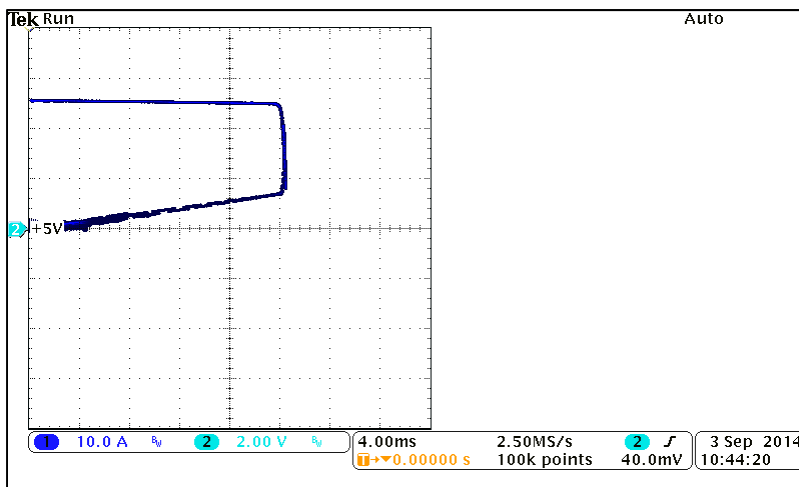
Figure 10: +5V Output over current characteristic
