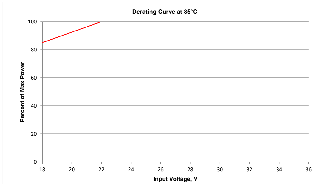
Figure 105: Derating curve for input voltage at 85°C
