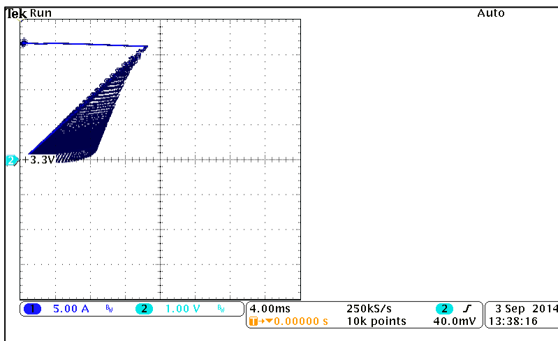
Figure 11: +3.3V Output over current characteristic
