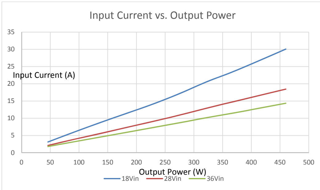
Figure 94: Input Current vs. Output Power
