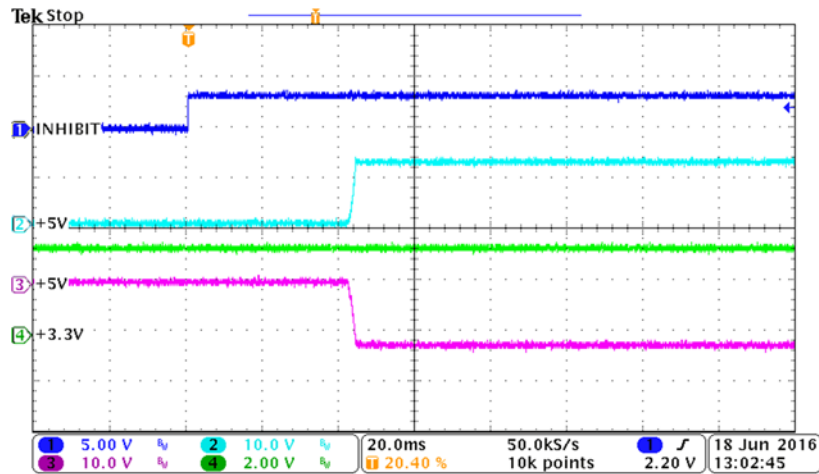
Figure 5: Turn-on delay from INHIBIT* de-assertion, auxiliary outputs
