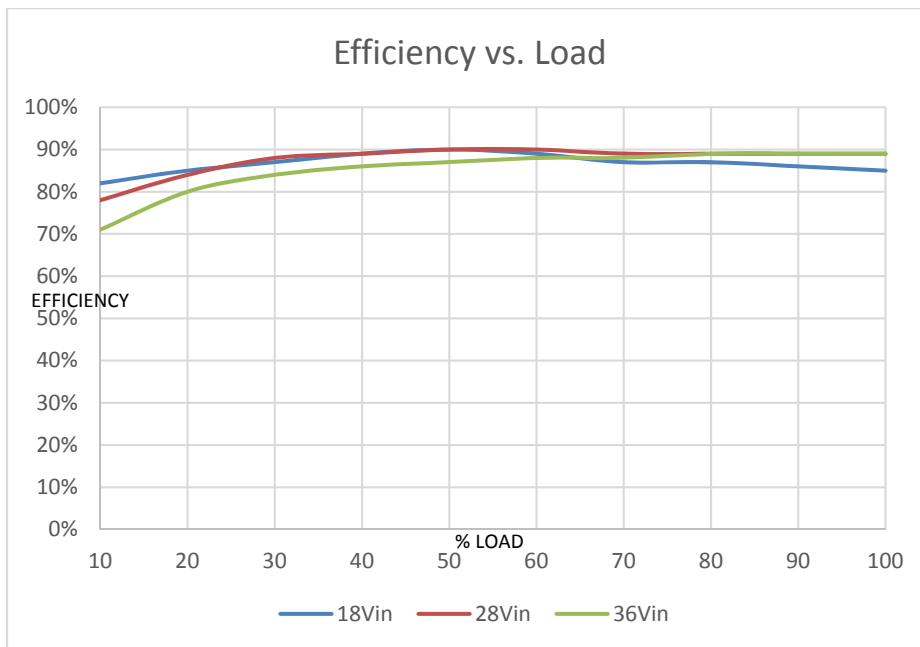
Figure 72: Efficiency vs. Load for Minimum, Nominal and Maximum input voltage
