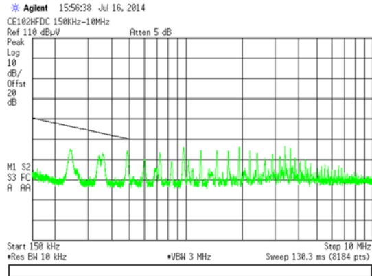
Figure 15: CE102 high frequency band scan
