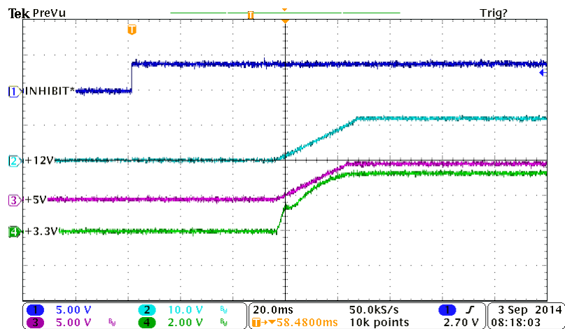
Figure 4: Turn-on delay from INHIBIT* de-assertion, main outputs
